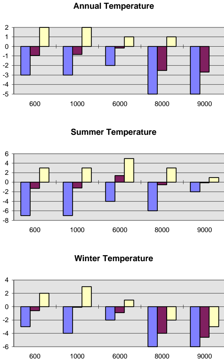
Figure 6.7b: Models of temperature in Minnesota, 600-9000 B.P., as compared to the present
